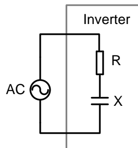
Series Connection
